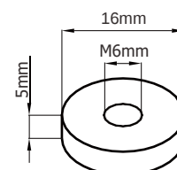
TERMINAL DIMENSION
